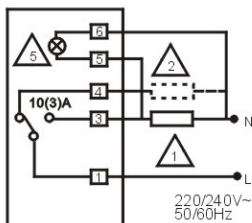
TR-010X(T6360A)
