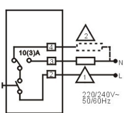
TR-001(T6360C)
